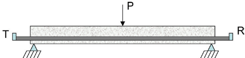
Figure 5-44: Reinforced beam is loaded by a transverse load P. Guided wave is sent from transmitter T to receiver R through the steel rod of this loaded beam.
