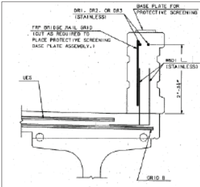
Figure 3-38: Section view of bridge rail connection to bridge deck
