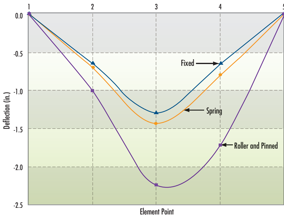
Figure 3-42: Quantification of bearing pad stiffness examples
