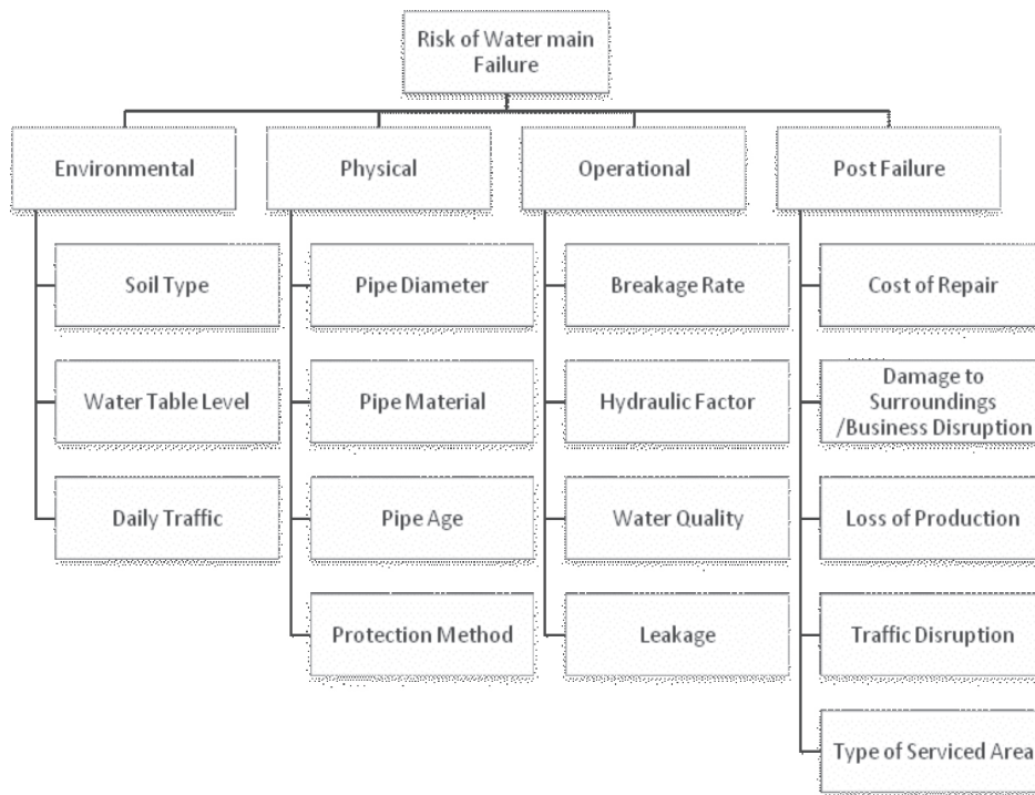
Figure 5-50: Hierarchical risk factors of water main failure
