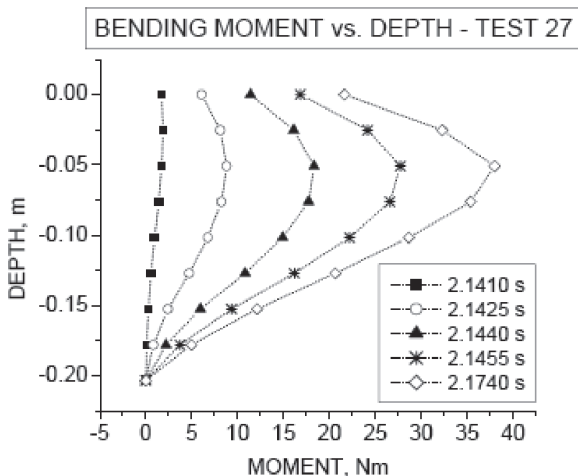
Figure 5-9: Bending Moment vs. Depth
