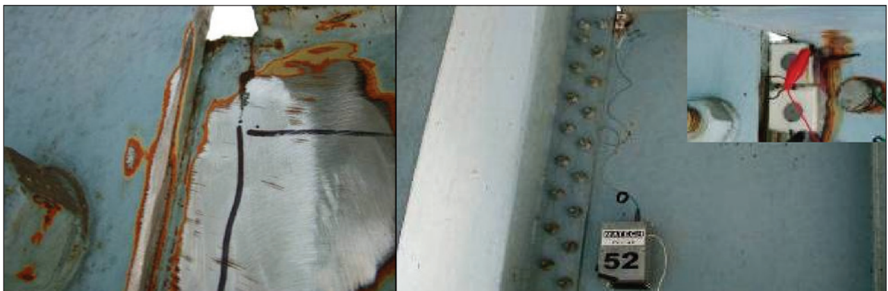
Figure 5-26: Typical cracked coped detail at the floor beam to girder connection. Photo on the right shows the detail with the EFS installed.
