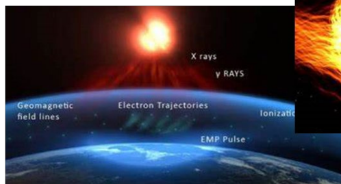
HEMP and GMD event examples
